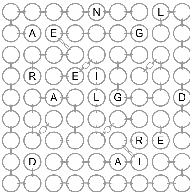
Chain-doku-2
